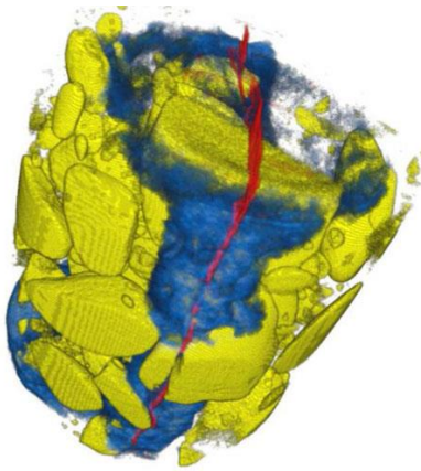
Concrete sample at the end of the injection test (yellow: gravels, red: initial crack, blue: wet zones)
