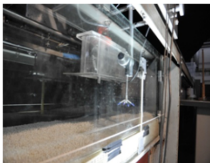
Sheet flow experiment at LEGI
