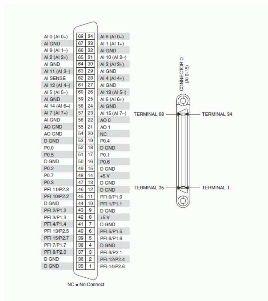
NI PCIe/PXIe-6341 Pinout
