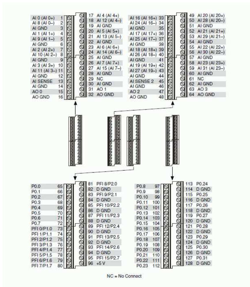
NI USB-6343 Pinout
