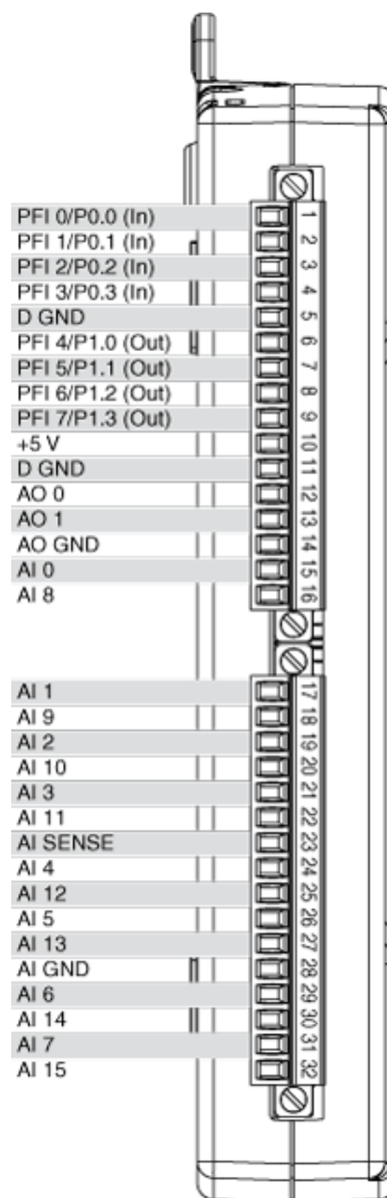
USB-6211/6215 Pinout
