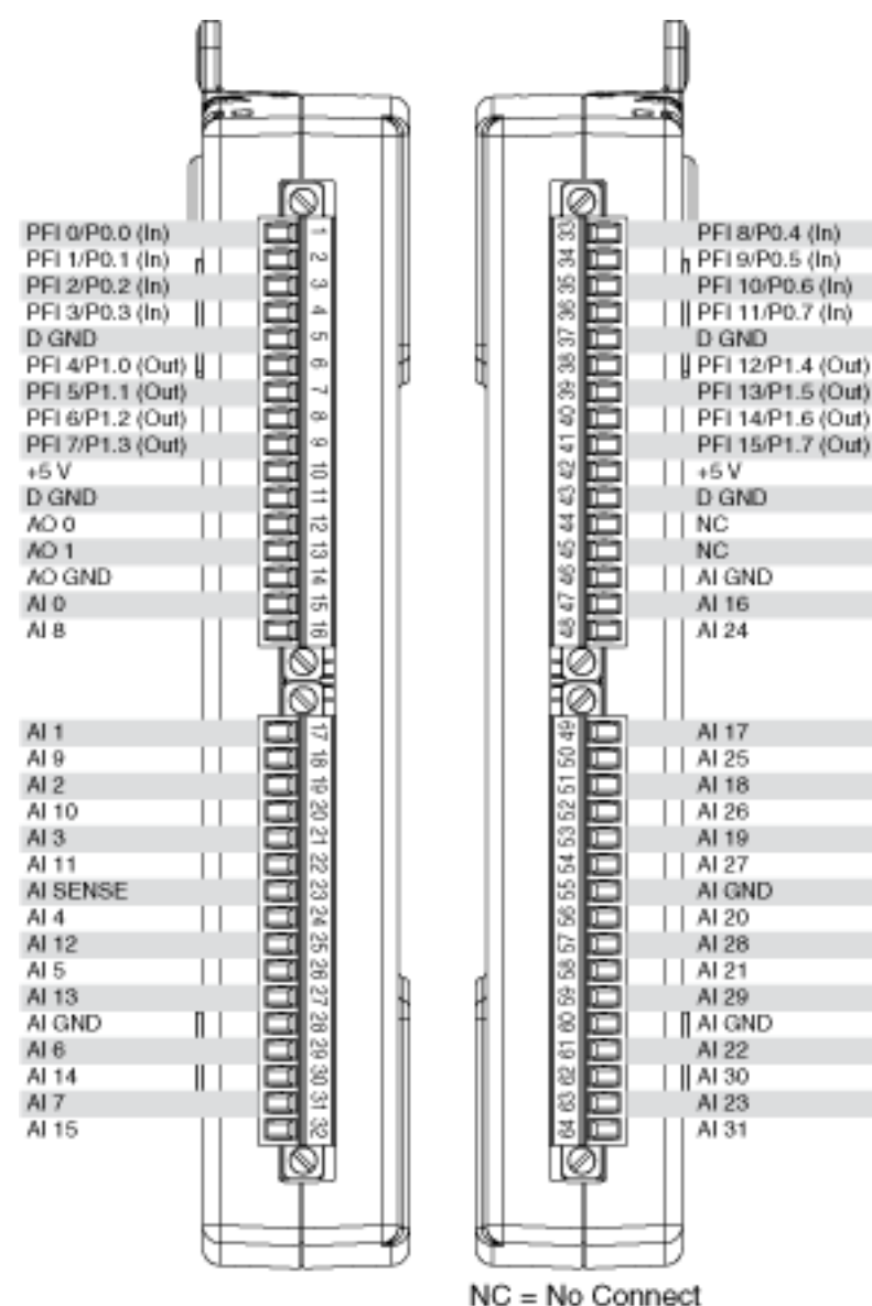
USB-6218 Pinout
