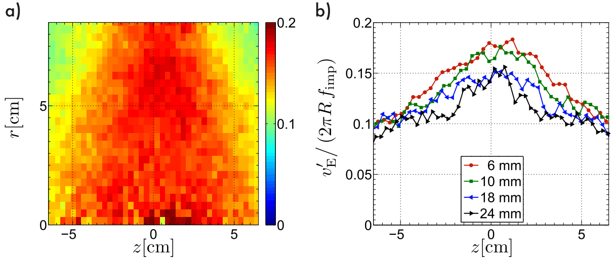
Figure 5. (a) Half cross section of the normalized fluctuating velocity v'_E(r, z)/(2\pi R f_{\text{imp}}) for 6 mm particles. (b) Longitudinal profile at r = 7 cm for increasing particle diameters. Data are from experiments at f_{\text{imp}} = 4 Hz.
